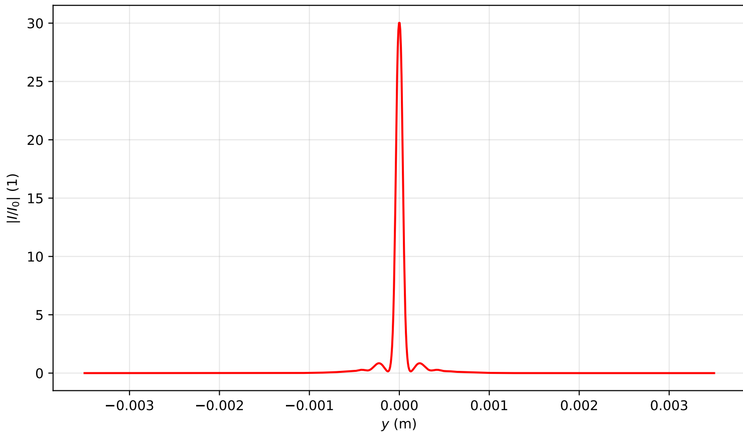
Intensity profile I(x=0, y, z=0.716)/I_0 , P_{in}=3.5P_{cr} , artificial time
